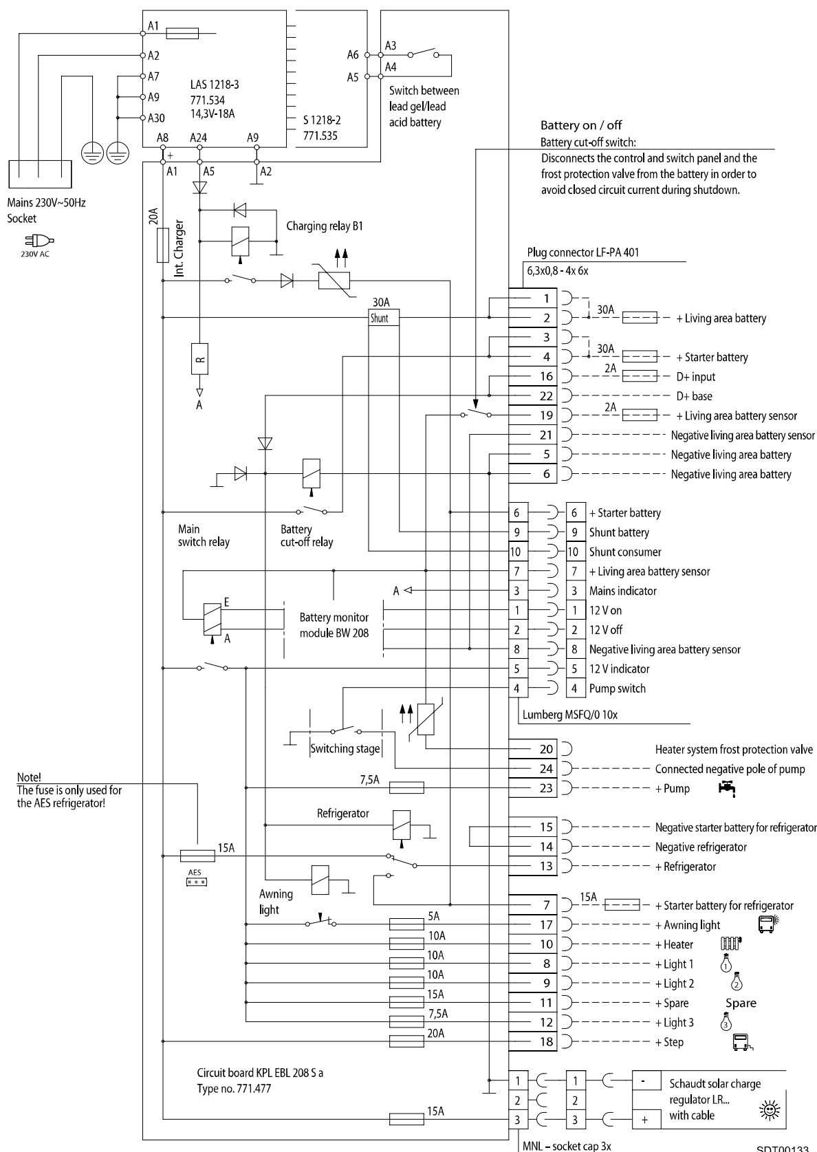
Fig. 2 Block diagram for Electrobloc EBL 208 S E
